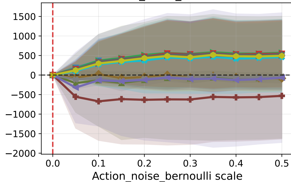
Action_noise_bernoulli
